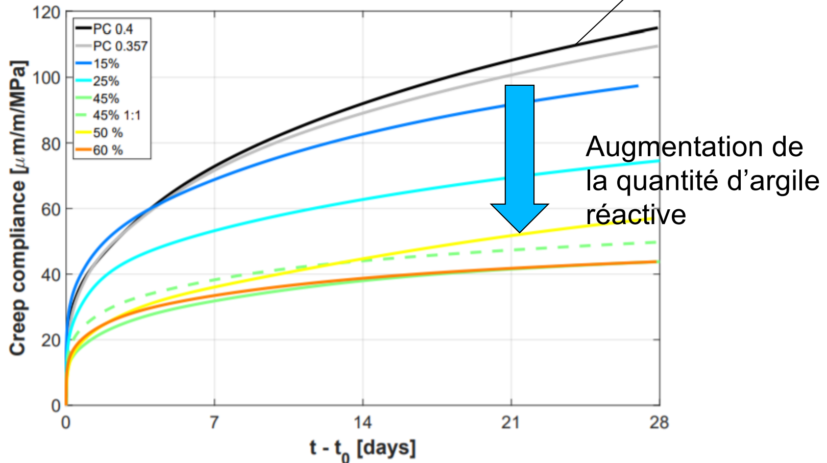
Figure 1.11 – Compressive creep compliance of the LC 3 -50 mixes, starting 28 days after casting.
